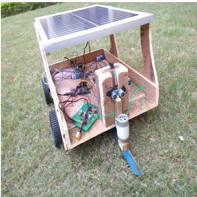
Automated Solar Lawn Mower
